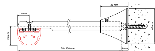
Wall mounting with adjustable extension bracket 6017
